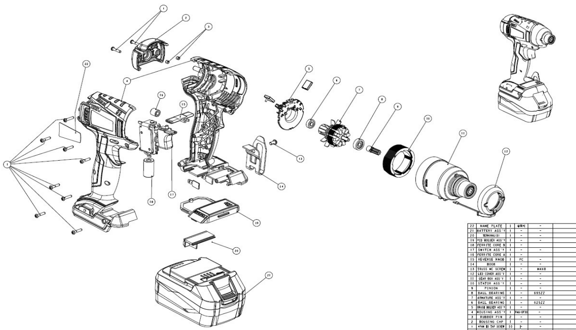
DIW-1801L EXPLODED VIEW(#8003809)
